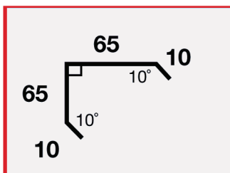
STD #13 150mm x 3 Fold Corner Flashing
