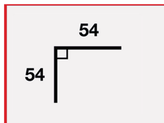
STD #14 450mm x 1 Fold Corner Flashing
