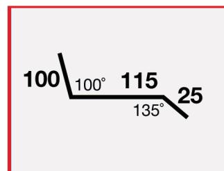
STD #7 240mm x 2 Fold Apron Flashing
