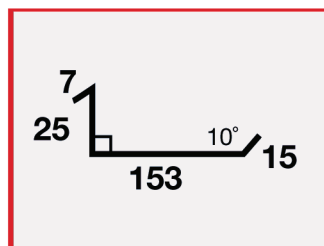
STD #6 200mm x 3 Fold Over Flashing
