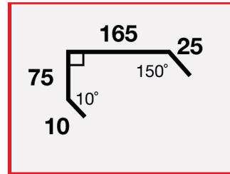
STD #3 275mm x 3 Fold Barge Capping
