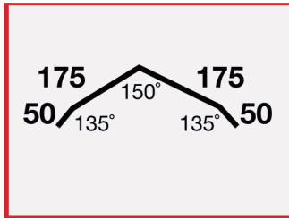
STD #1 450mm x 3 Fold Vee Ridge
