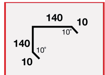
STD #12 300mm x 3 Fold Corner Flashing
