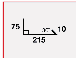
STD #11 450mm x 2 Fold Soaker Flashing
