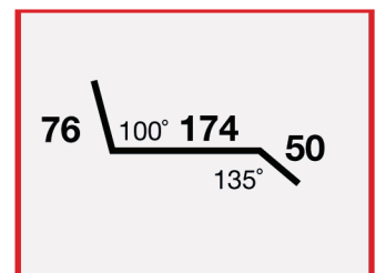
STD #8 300mm x 2 Fold Apron Flashing
