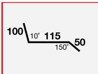
STD #9 265mm x 2 Fold Apron Flashing
