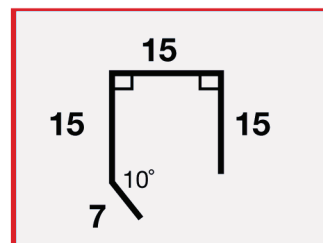
Rolclad® FENCE CAPPING Zincalume®™
