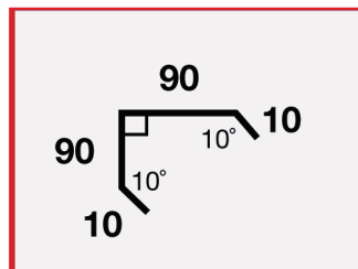
STD #10 200mm x 3 Fold Corner Flashing
