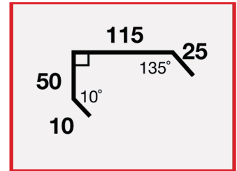
STD #4 200mm x 3 Fold Barge Capping
