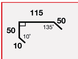
STD #5 225mm x 3 Fold Barge Capping
