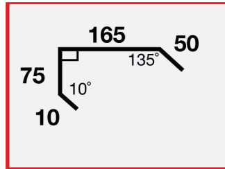
STD #2 300mm x 3 Fold Barge Capping
