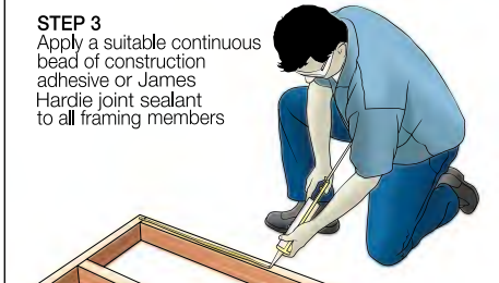
FIGURE 3 CONSTRUCTION ADHESIVE
