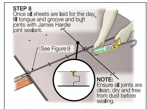
FIGURE 10 SEALING ALL JOINTS
