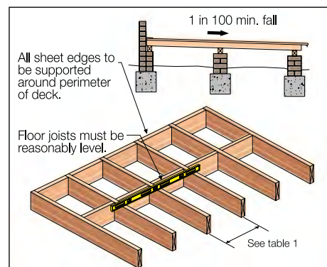
FIGURE 1 FRAME PREPARATION
